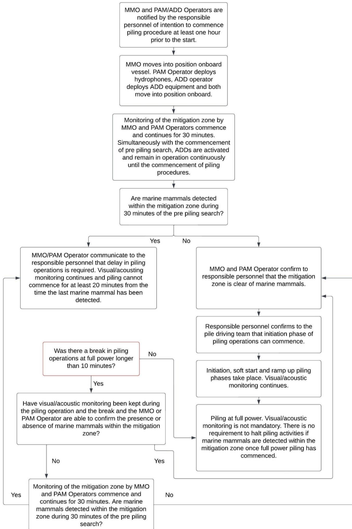
Figure 1.2: Piling mitigation.
